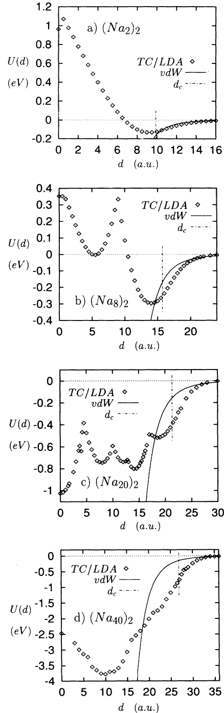
FIG. 2. U_{\text{TC/LDA}}(d) from Eq. (1) (TC/LDA) in comparison to U_{\text{vdW}}(d) from Ref. 7: (a) (\text{Na}_2)_2 ; (b) (\text{Na}_8)_2 ; (c) (\text{Na}_{20})_2 ; (d) (\text{Na}_{40})_2 . The vertical line indicates the contact point d_c of the two \text{Na}_N clusters.
