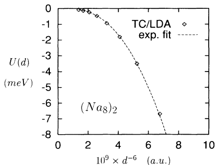
FIG. 1. Asymptotic form of U_{\text{TC/LDA}}(d) compared with an exponential fit as a function of d^{-6} . Note that for obtaining U_{\text{TC/LDA}}(d) for each d the two-center energy E[(\text{Na}_8)_2](d) and the single-cluster energy E[\text{Na}_8] have been calculated using the two-center code with identical basis sets, thus reducing the error in U_{\text{TC/LDA}}(d) due to basis set truncation by about one order of magnitude. The largest discrepancy between the E[\text{Na}_8] evaluated in this way and a fully numerical one-center calculation is 0.18 meV (for d = 30 a.u.).
