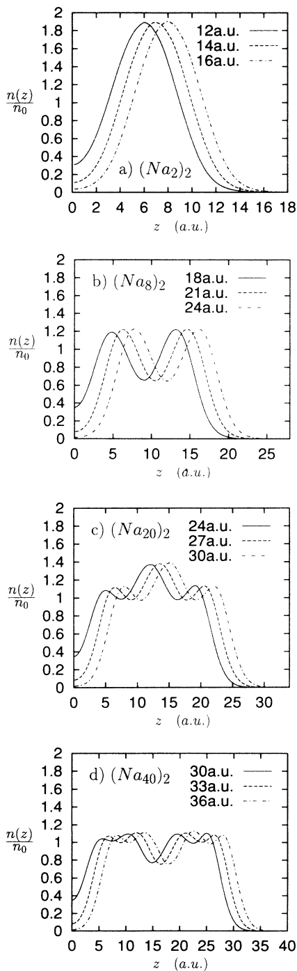
FIG. 3. Density profiles along the symmetry axis (normalized to the bulk value n_0 ) at different intercluster separations: (a) (\text{Na}_2)_2 ; (b) (\text{Na}_8)_2 ; (c) (\text{Na}_{20})_2 ; (d) (\text{Na}_{40})_2 .
